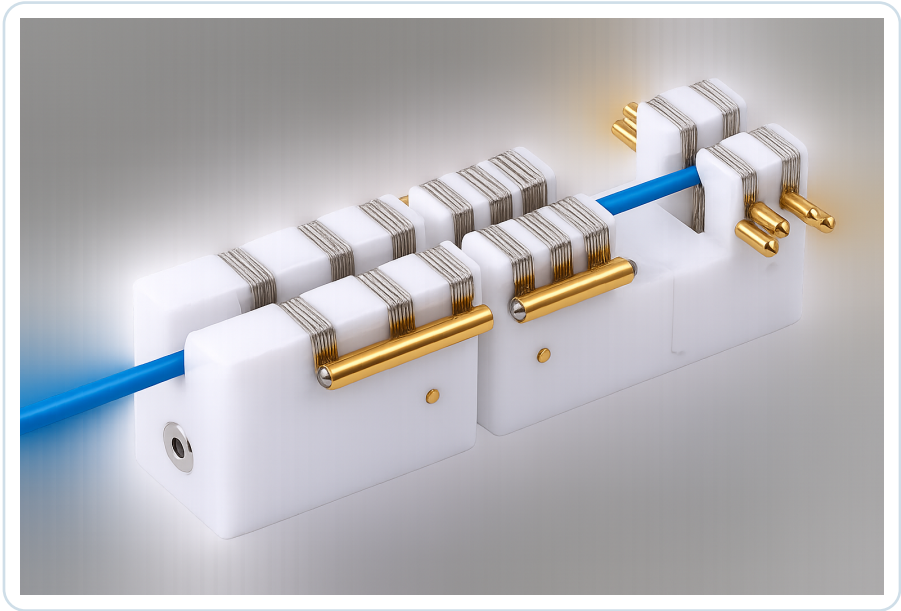
Contact Modules A, B and C shown assembled on catheter shaft
